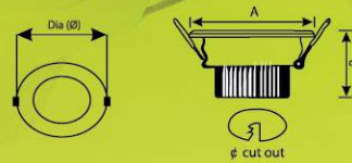
MDLCOB 01 3/7/10/15/20/30 W
